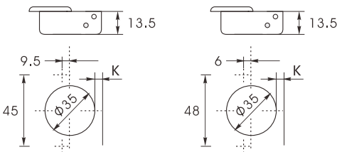
铰杯种类 Hinge cup types
