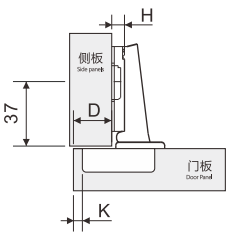
full overlay
