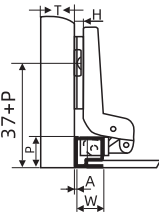
inset
