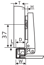
full overlay
