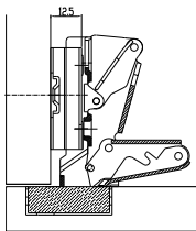
full overlay
