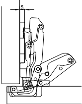
half overlay
