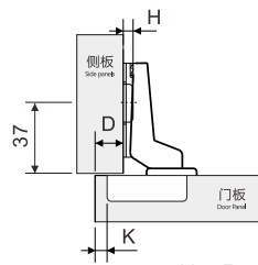
half overlay
