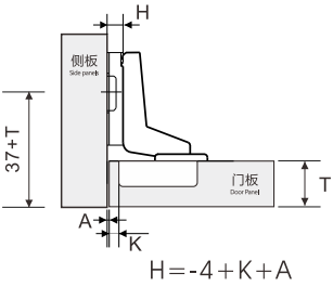
inset
