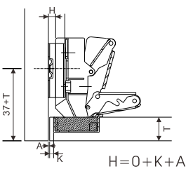
inset
