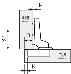
half overlay
