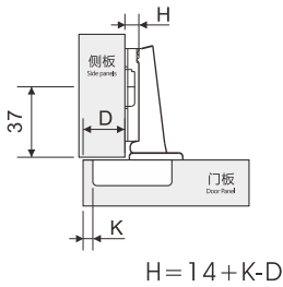
full overlay
