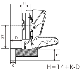
full overlay
