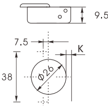
铰杯种类 Hinge cup types
