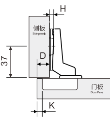
half overlay
