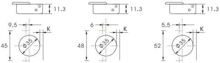
铰杯种类 Hinge cup types
