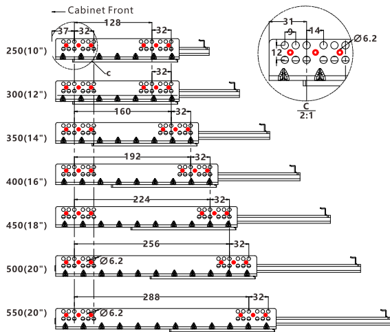
滑轨安装孔位 Mounting Hole Position
