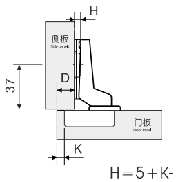
half overlay
