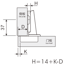
full overlay
